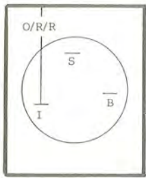
BACKSIDE OF IGNITION SWITCH
