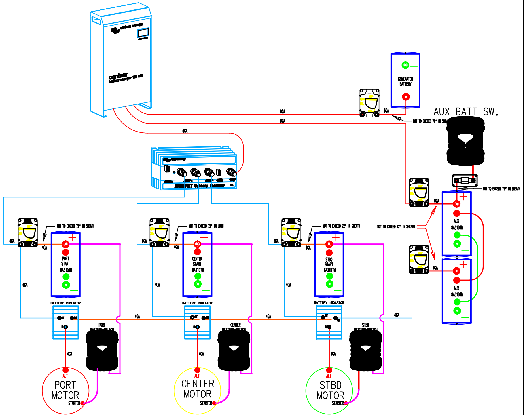
MERCURY TRIPLE OB ENGINE
