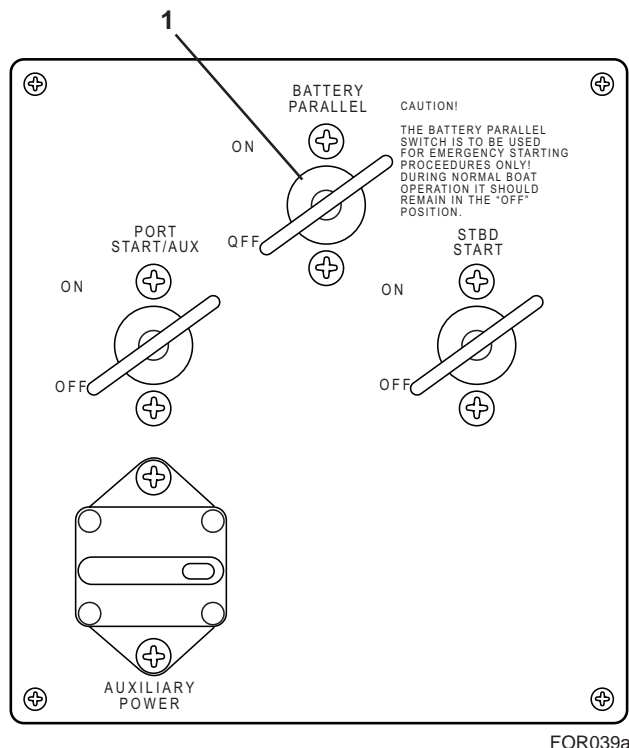
Typical Twin Engine Battery Switch Figure 4-34
