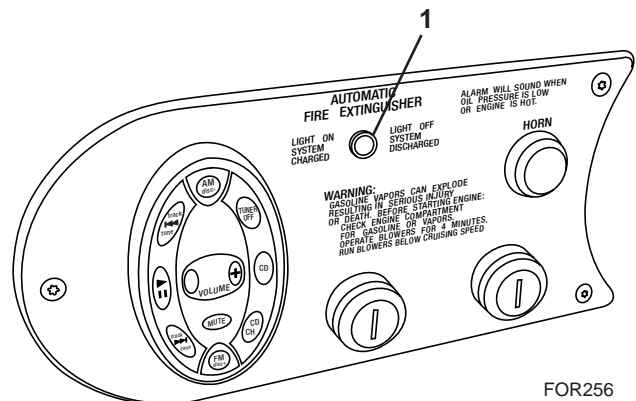
1. Indicator Light
