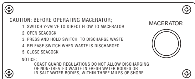
Macerator Control Panel Figure 4-32
