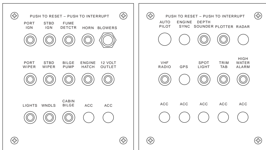
Typical Circuit Breaker Panel Figure 4-17
