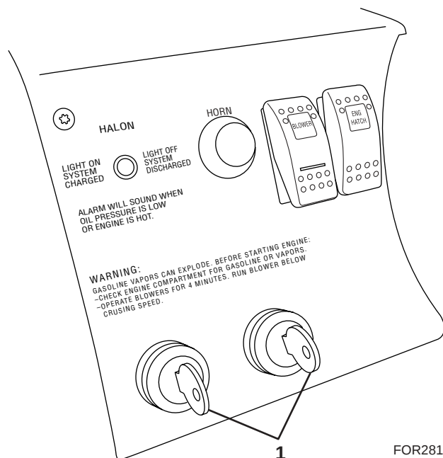
1. Ignition Switches
