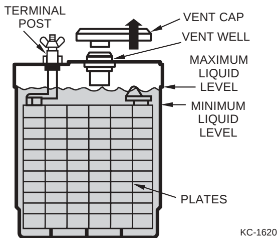
Battery Figure 9-1
