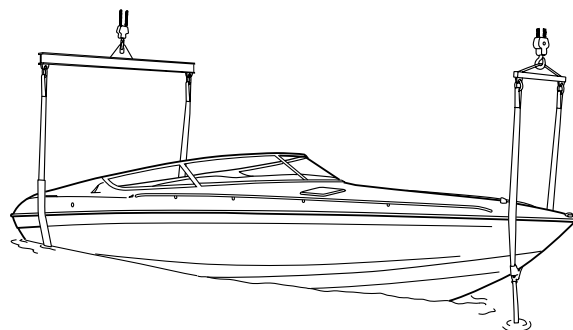
Lifting with Slings Figure 10-1
