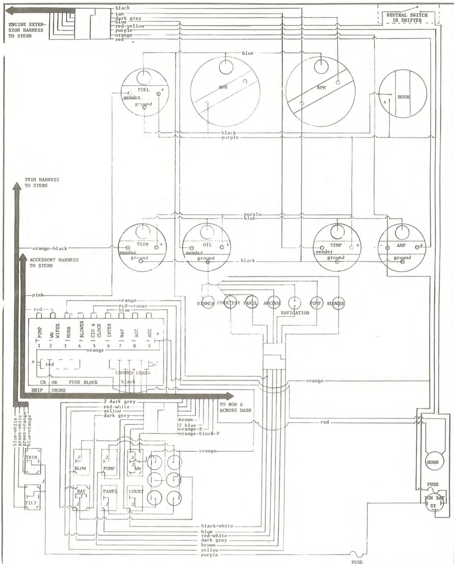
F233 HARDTOP, COASTAL, CUDDY, REAR DASH VIEW, SINGLE OMC ENGINE. P = PORT, S = STAR- BOARD, J = JUMPER 20D
