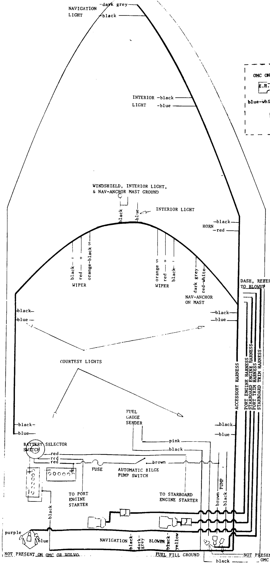
BOAT WIRING LAYOUT
