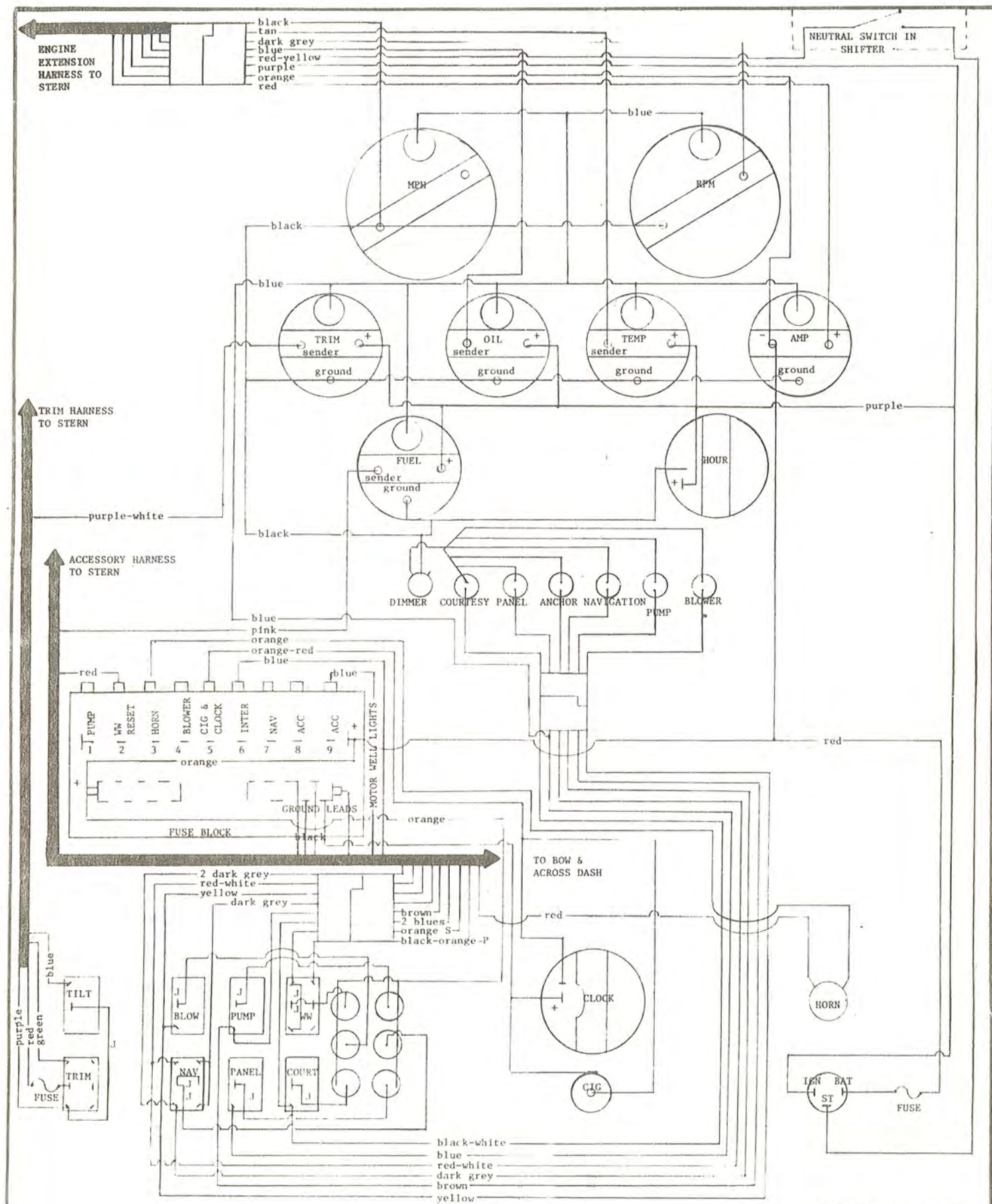
F255 CASTAWAY, REAR DASH VIEW, SINGLE MERCURY ENGINE P = PORT, S = STARBOARD J = JUMPER
