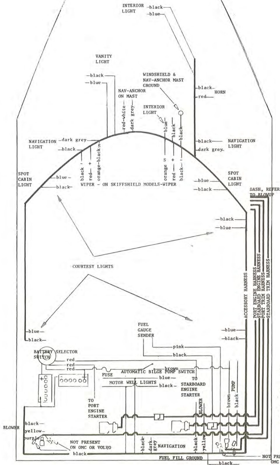
BOAT WIRING LAYOUT
