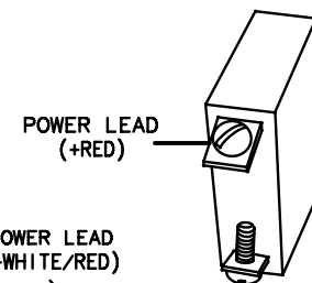
ENGINE HATCH BREAKER (DASH BREAKER PANEL) (REAR VIEW)
