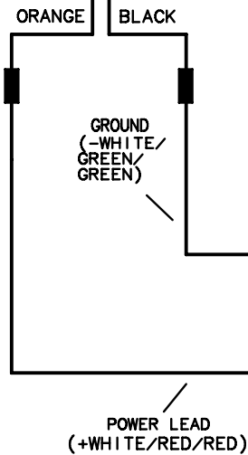
ENGINE HATCH SWITCH (DASH PANEL) (REAR VIEW)
