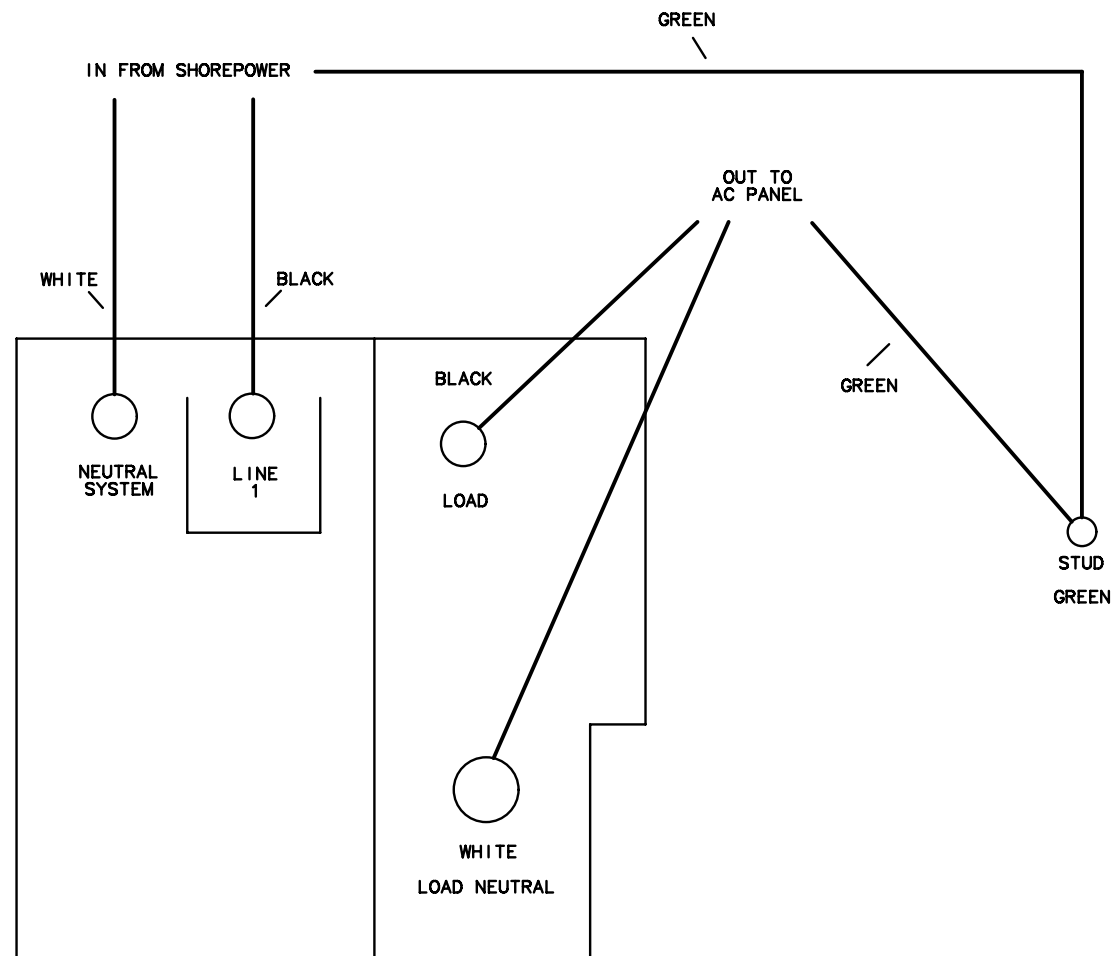
SHOREPOWER ELCI BREAKER (REAR VIEW) (LOCATED UNDER THE AFT PORT LOUNGE SEAT)
