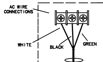
DETAIL VIEW (CONNECTIONS INSIDE)
