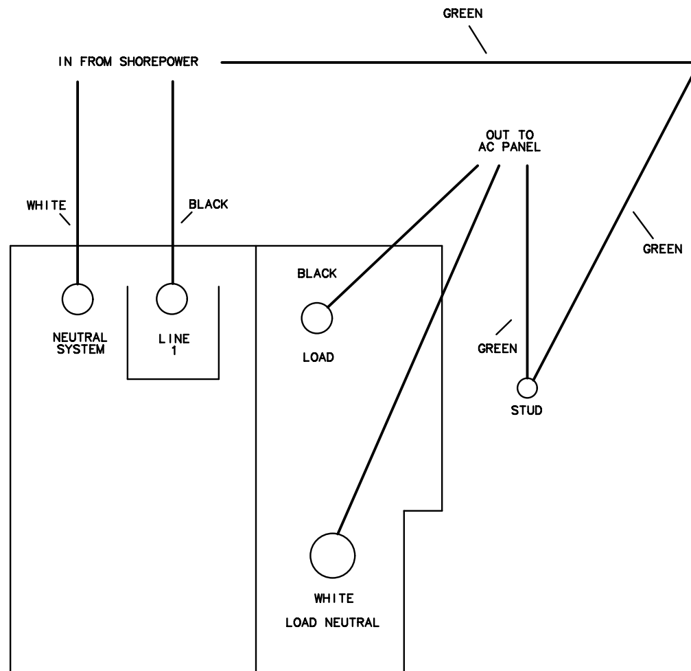
SHOREPOWER ELCI BREAKER (REAR VIEW) (LOCATED UNDER THE AFT CORNER STARBOARD LOUNGE SEAT)
