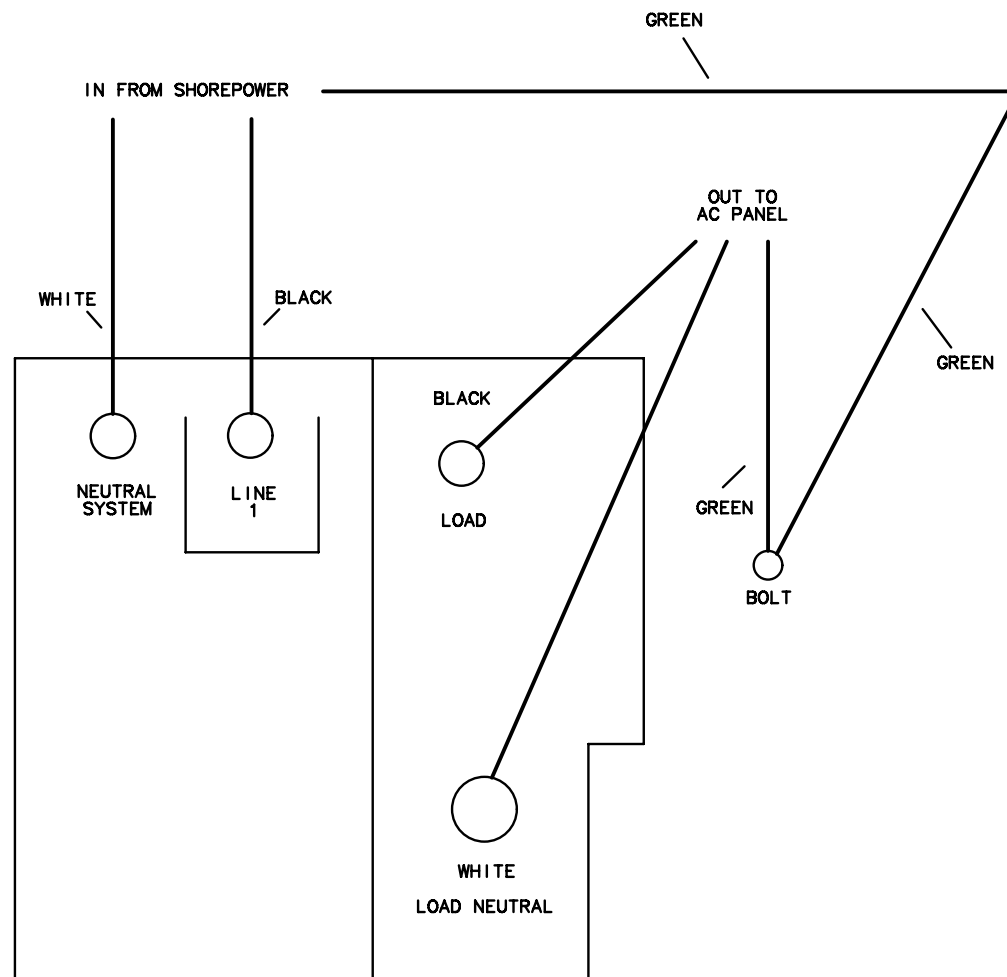
SHOREPOWER BREAKER (REAR VIEW) (LOCATED UNDER THE AFT CORNER STARBOARD LOUNGE SEAT)
