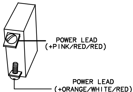
HIGH WATER ALARM BREAKER AFT BREAKER PANEL (REAR VIEW)
