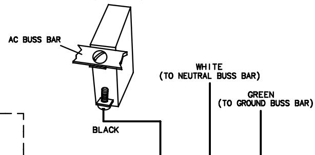
BATTERY CHARGER BREAKER (120V AC SYSTEMS PANEL) (REAR VIEW)
