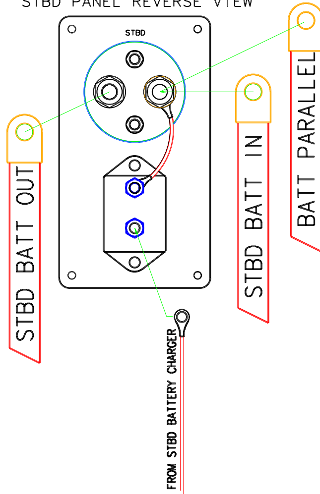
STBD PANEL REVERSE VIEW
