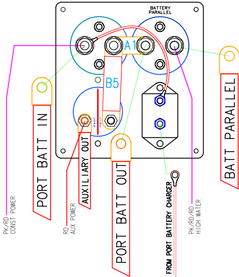
PORT PANEL REVERSE VIEW
