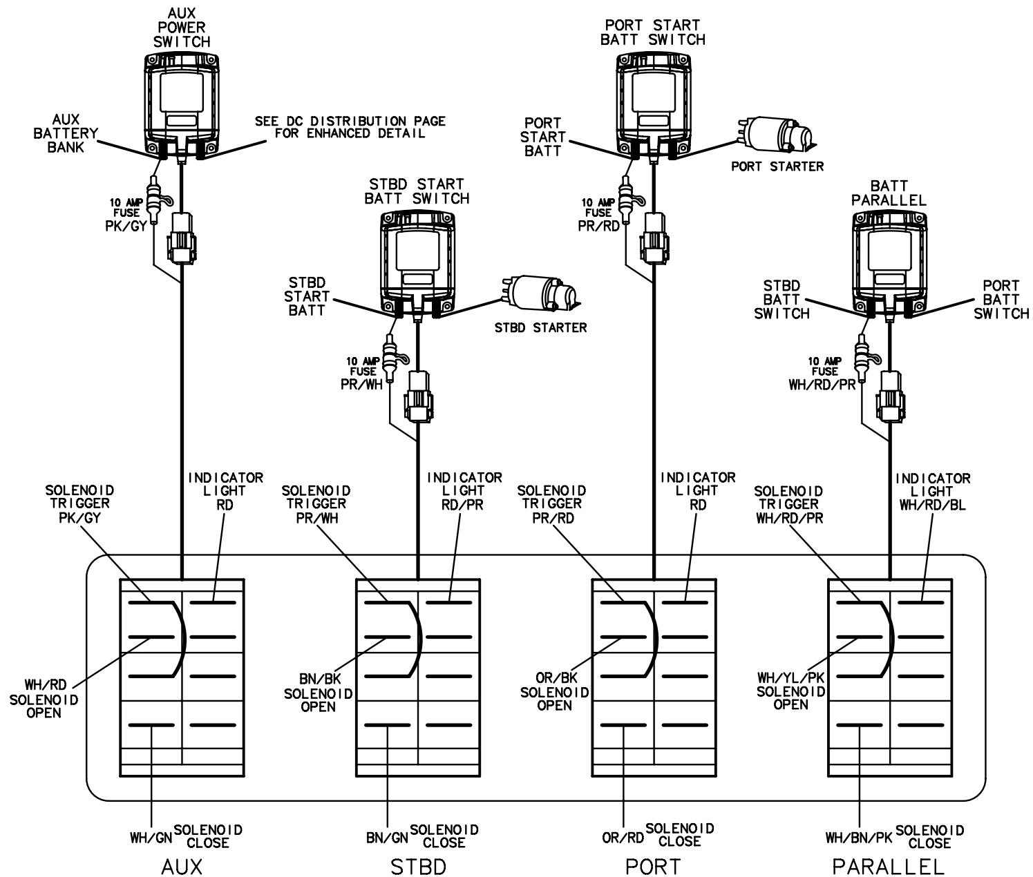
BATTERY SWITCH PANEL (REAR VIEW)
