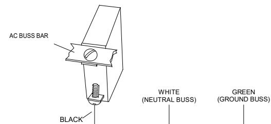
BATTERY CHARGER BREAKER (120/240V AC SYSTEMS PANEL)
