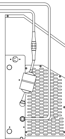
KRA UNIT (SIDE VIEW)
