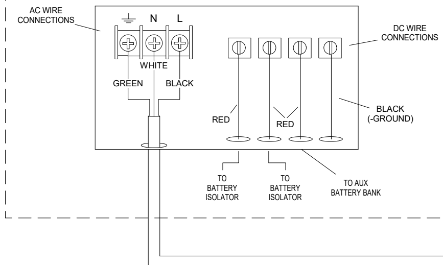
DETAIL VIEW (CONNECTIONS INSIDE)
